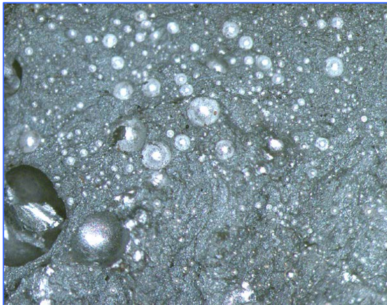
Macrograph showing gas porosity
