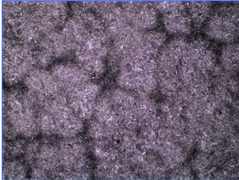
Micrograph showing chemical segregation in a steel casting
