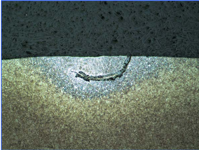
Micrograph of a forging lap
