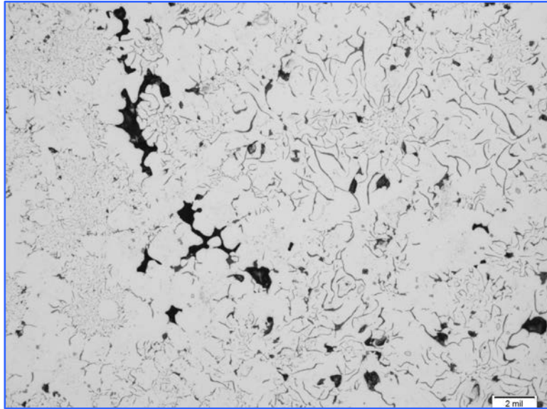
Micrograph showing shrinkage voids in cast iron
