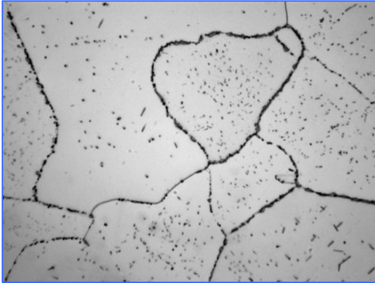
Microstructure showing the onset of incipient melting at the grain boundaries
