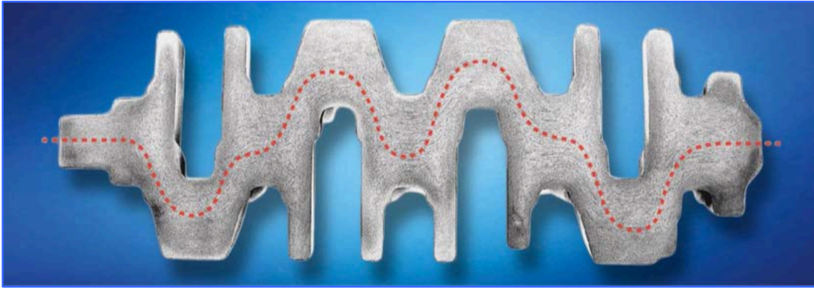
Section of a crankshaft showing the desirable grain flow pattern produced during forging
